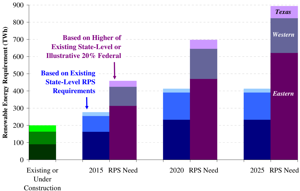
Figure 12 Cumulative Renewable Energy Need (TWh)
