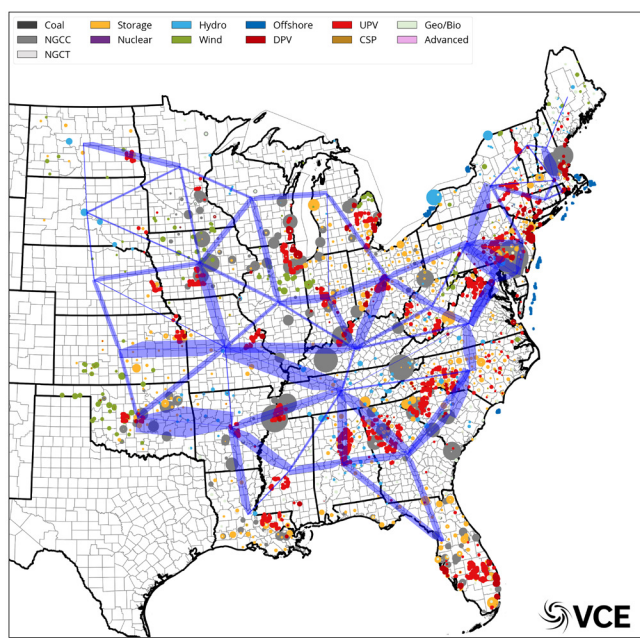
Figure 35: Weak carbon, high wind deployment, 2050
