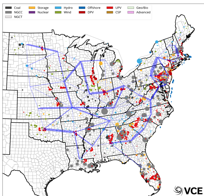
Figure 31: Weak carbon, high wind deployment, 2030
