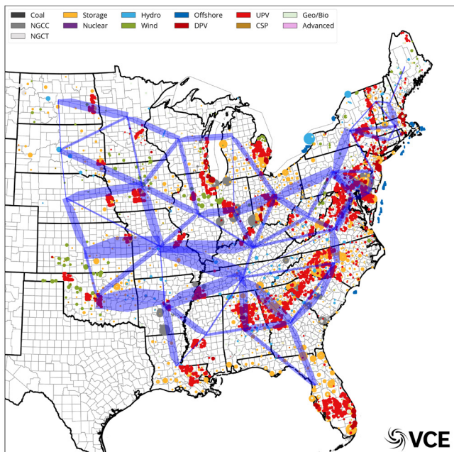
Figure 33: Strong carbon, high wind deployment, 2050
