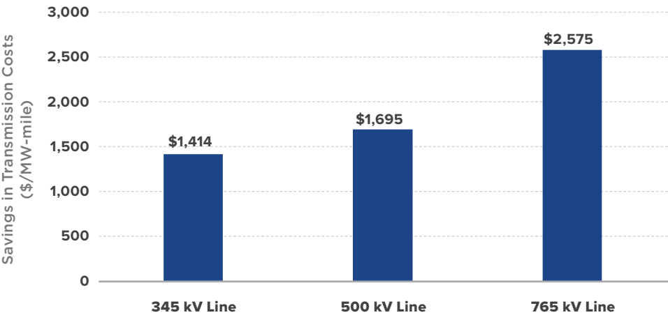
FIGURE 7 Savings from deploying high-capacity transmission compared to 230 kV transmission lines Data Source: MISO 27
